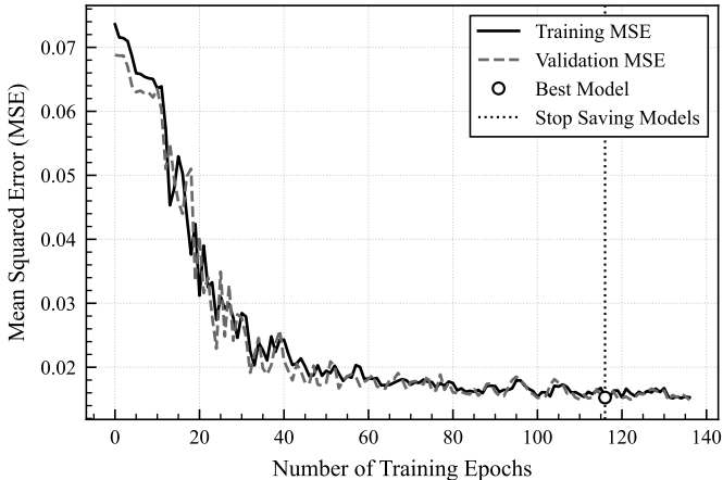
Learning Curve of MHSA-GRU Model for SolarPlant-2 (Gyeongju)
